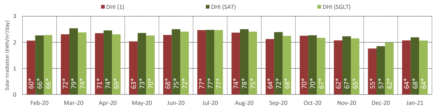
*Monthly Total Irradiation (kWh/m 2 /month)
